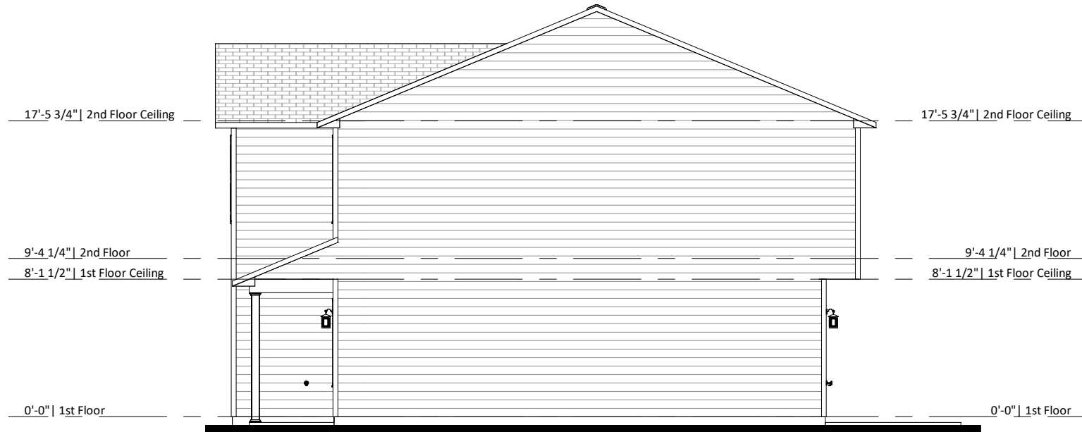
② Right Elevation - Elev A - 1 Car Garage 1/8" = 1'-0"
