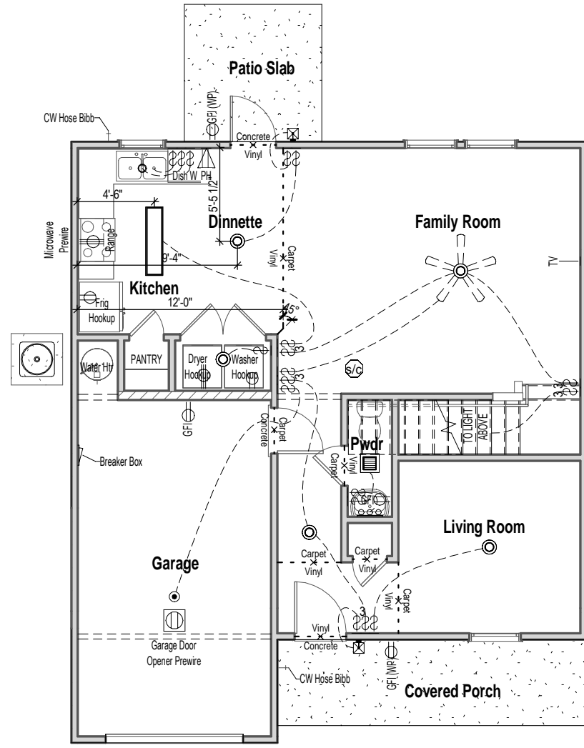
① 1st Floor Electrical - Elev A - 1 Car Garage 1/8" = 1'-0"
