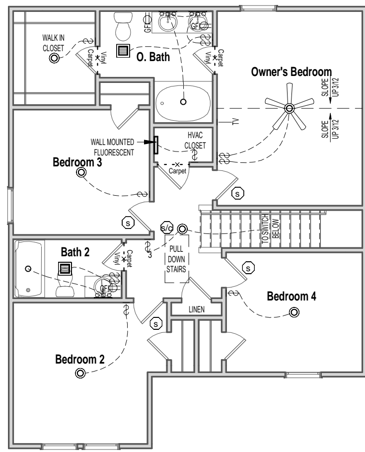
② 2nd Floor Electrical - Elev A - 1 Car Garage 1/8" = 1'-0"
